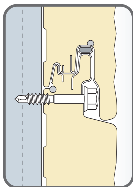
External: Typical engineered joint
